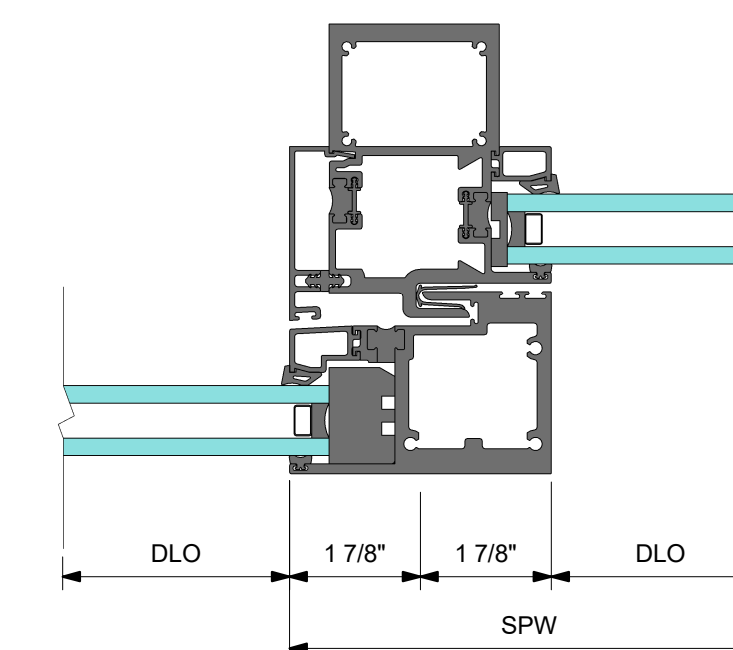
6 DETAIL 6 VERTICAL OX INTERMEDIATE FIXED SLIDING WITH STANDARD INTERLOCK
