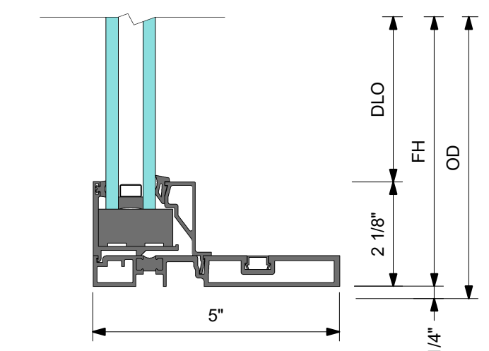
4 DETAIL 4 LOW PROFILE SILL AT FIXED PANEL
