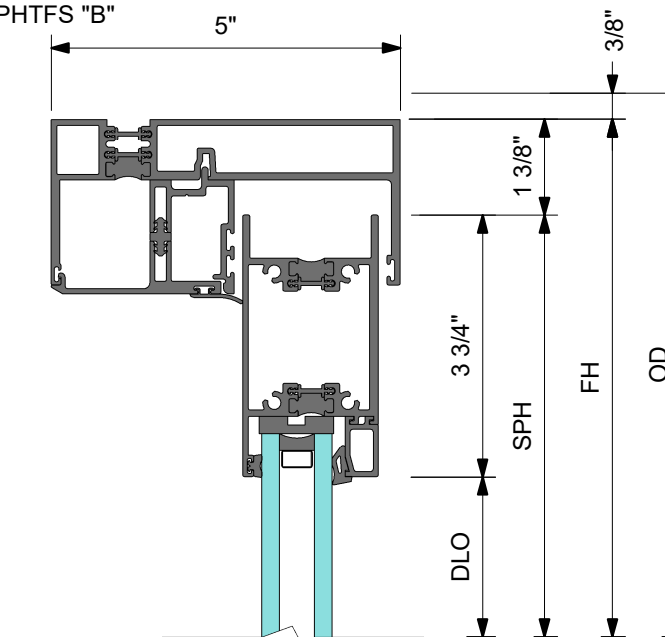
1 DETAIL 1 HEAD AT SLIDING PANEL
