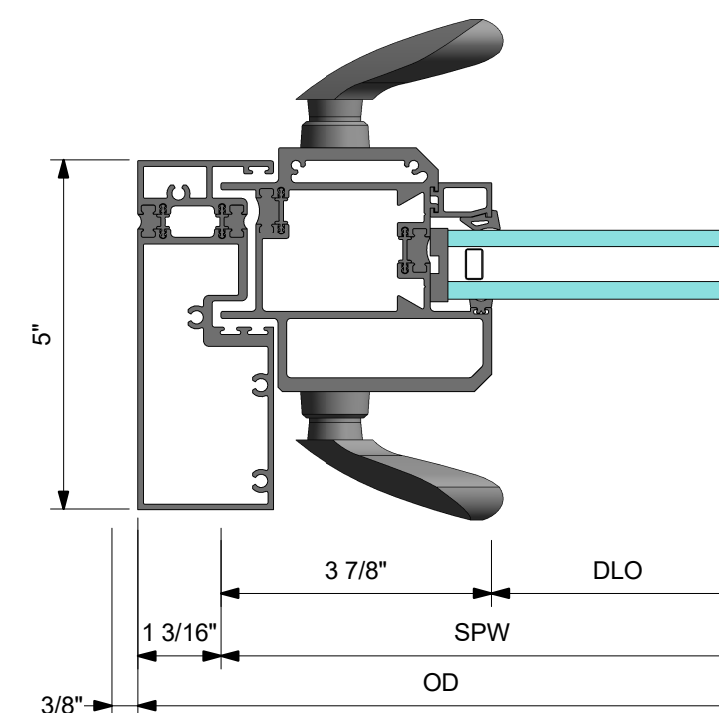
5 DETAIL 5 VERTICAL XO JAMB WITH STANDARD PULL SLIDING PANEL STILE
