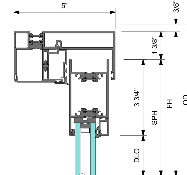
1 DETAIL 1 HEAD AT SLIDING PANEL
