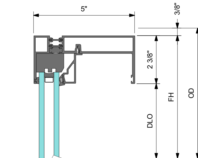
2 DETAIL 3 HEAD AT FIXED PANEL
