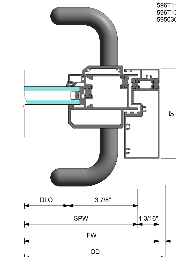
7 DETAIL 7 VERTICAL OX JAMB WITH CO-9 PULL SLIDING PANEL STYLE
