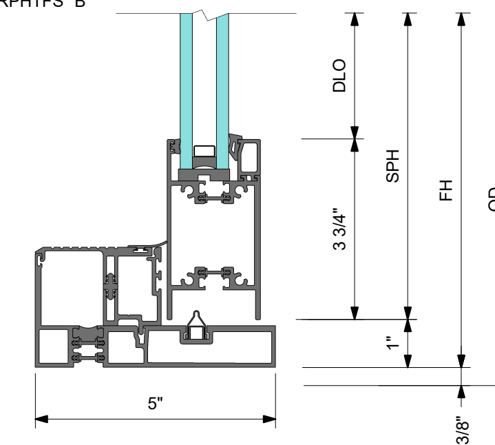
2 DETAIL 2 SILL AT SLIDING PANEL
