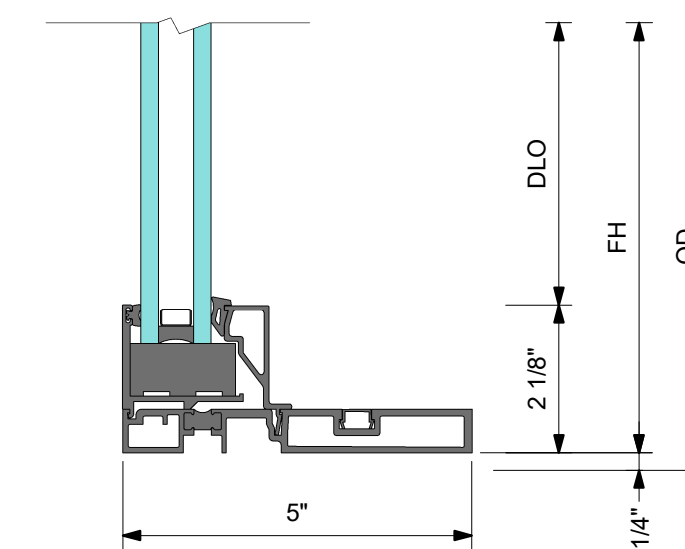
4 DETAIL 4 LOW PROFILE SILL AT FIXED PANEL
