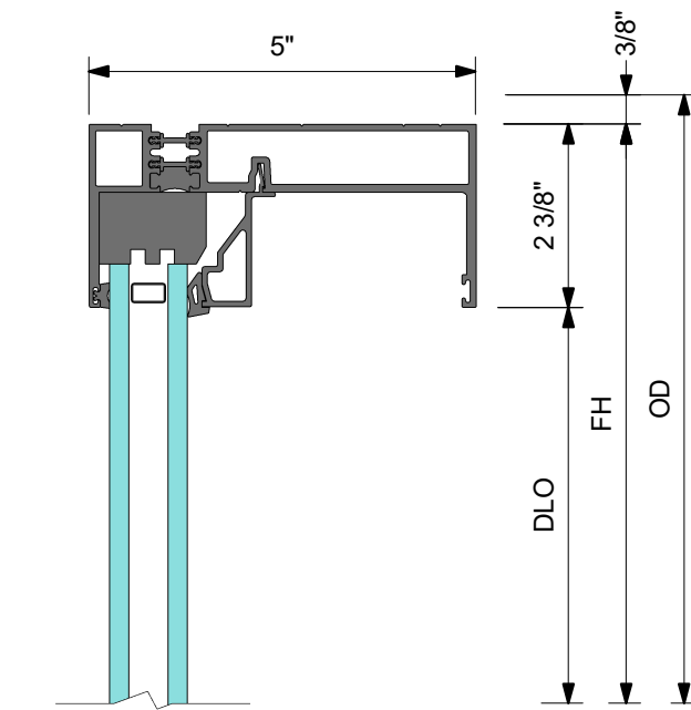
3 HEAD AT FIXED PANEL
