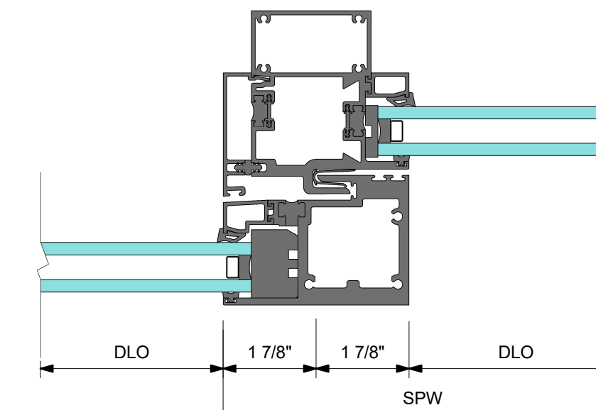
6 DETAIL 6 VERTICAL OX INTERMEDIATE FIXED SLIDING WITH STANDARD INTERLOCK
