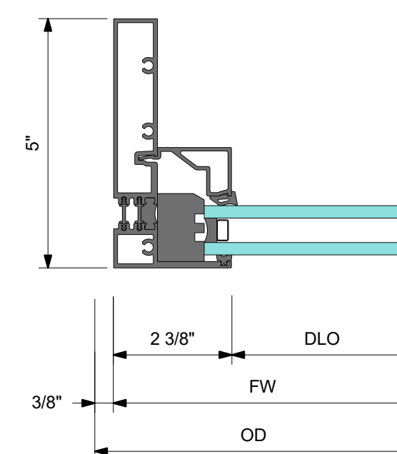
5 DETAIL 5 VERTICAL OX JAMB FIXED PANEL
