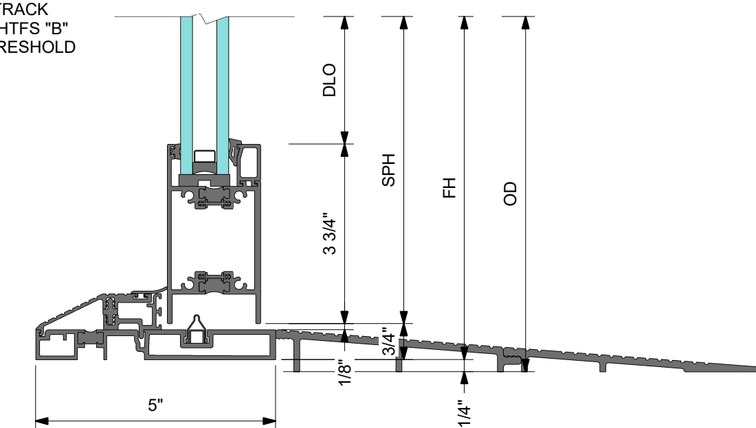
2 DETAIL 2 LOW PROFILE SILL WITH RAMP AT SLIDING PANEL
