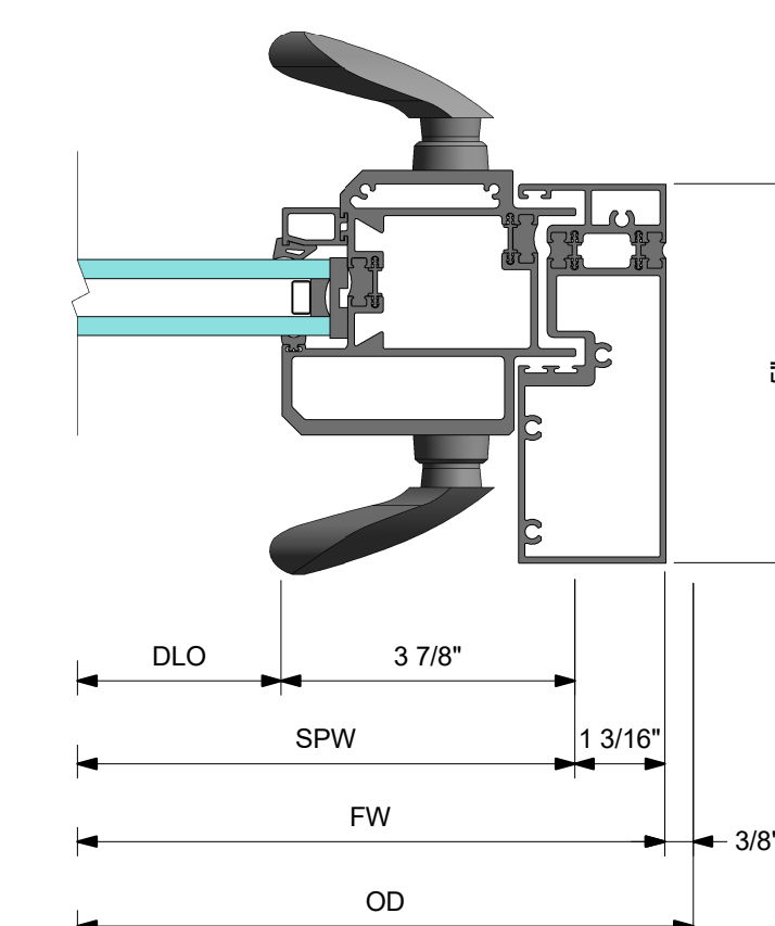
7 DETAIL 7 VERTICAL OX JAMB WITH STANDARD PULL SLIDING PANEL STILE
