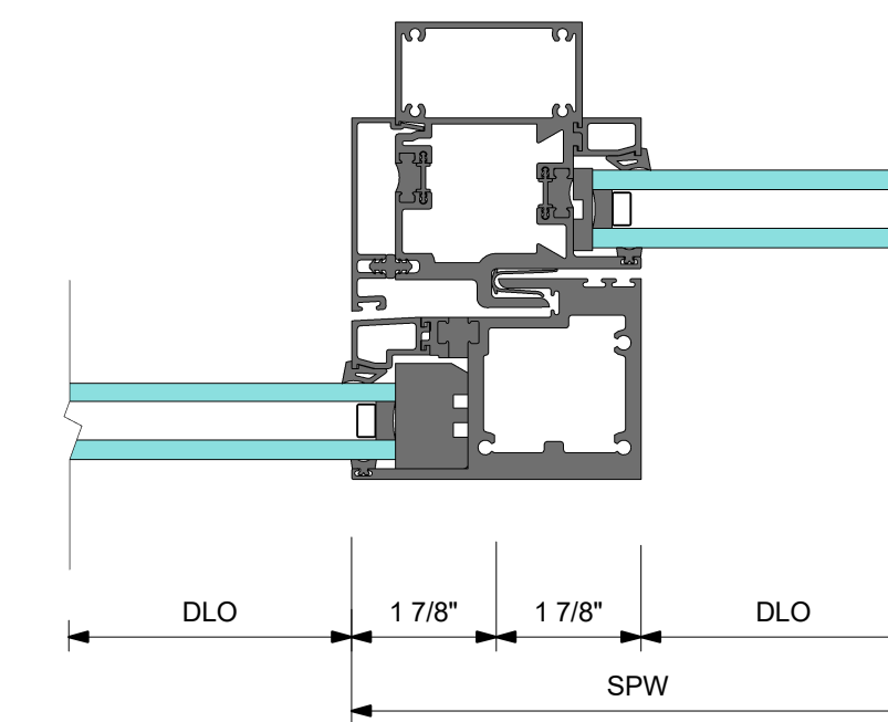
6 DETAIL 6 VERTICAL OX INTERMEDIATE FIXED SLIDING WITH STANDARD INTERLOCK
