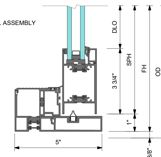
2 DETAIL 2 SILL AT SLIDING PANEL
