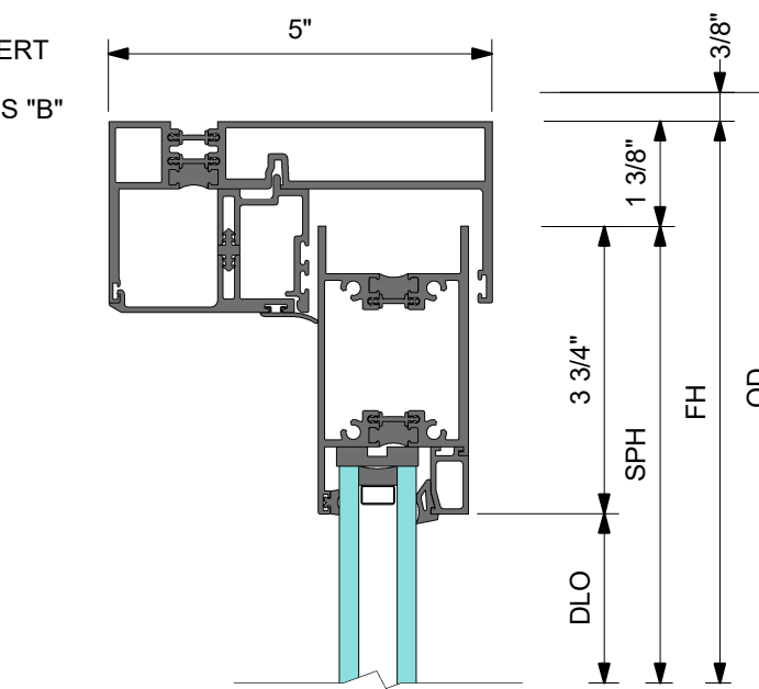
1 DETAIL 1 HEAD AT SLIDING PANEL
