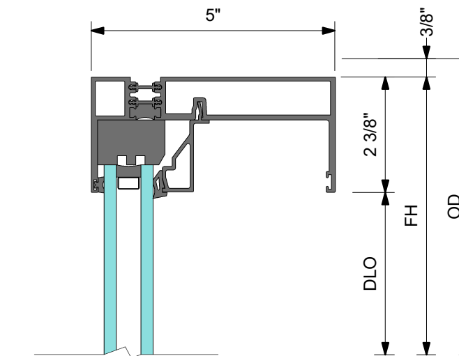
3 DETAIL 3 HEAD AT FIXED PANEL
