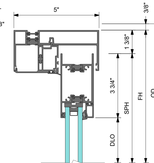
1 DETAIL 1 HEAD AT SLIDING PANEL
