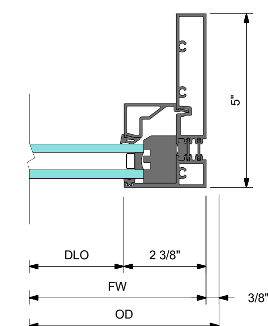
7 DETAIL 7 VERTICAL XO JAMB FIXED PANEL
