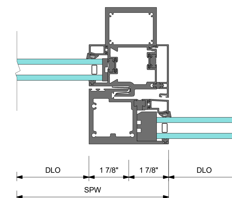
6 DETAIL 6 VERTICAL XO INTERMEDIATE FIXED SLIDING WITH STANDARD INTERLOCK
