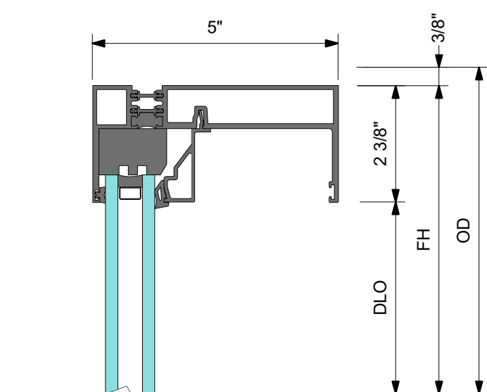
3 DETAIL 3 HEAD AT FIXED PANEL
