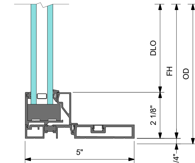
4 LOW PROFILE SILL AT FIXED PANEL
