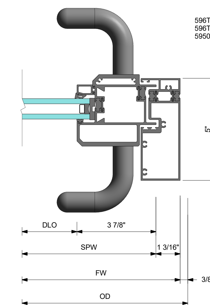
7 DETAIL 7 VERTICAL OX JAMB WITH CO-9 PULL SLIDING PANEL STYLE
