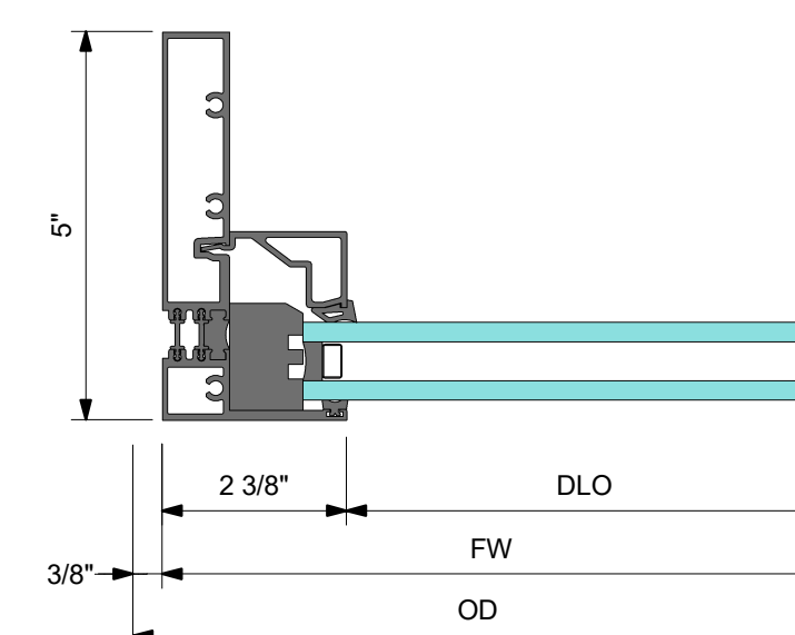
5 DETAIL 5 LOW PROFILE SILL AT FIXED PANEL
