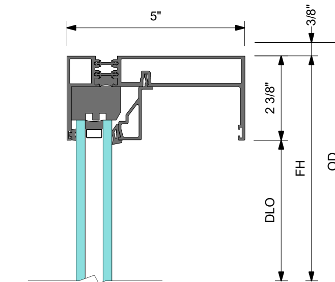
3 DETAIL 3 HEAD AT FIXED PANEL
