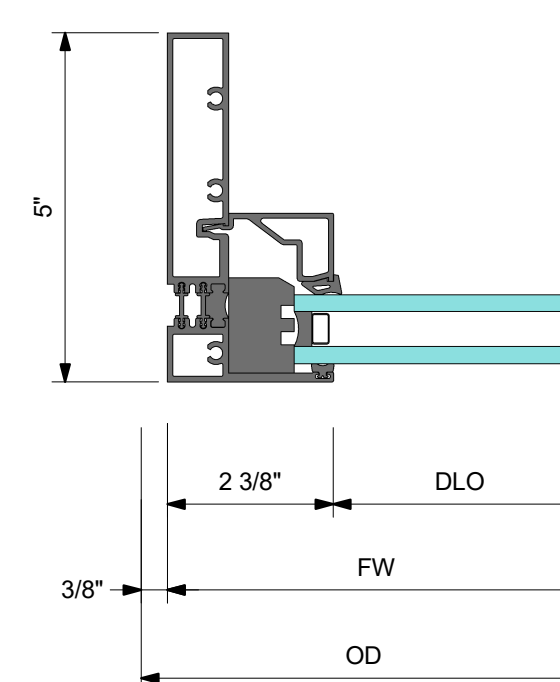
5 DETAIL 5 VERTICAL OX JAMB FIXED PANEL
