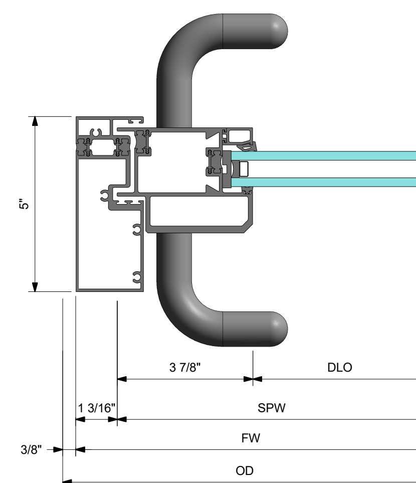
5 DETAIL 5 VERTICAL XO JAMB WITH CO-9 PULL SLIDING PANEL STILE
