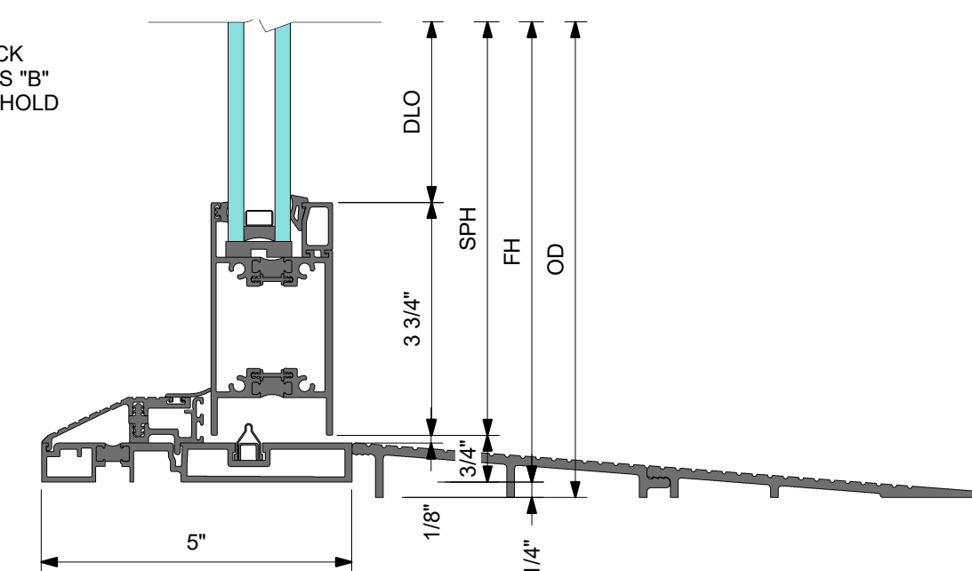
3 DETAIL 2 LOW PROFILE SILL WITH RAMP AT SLIDING PANEL
