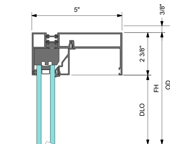
2 DETAIL 3 HEAD AT FIXED PANEL
