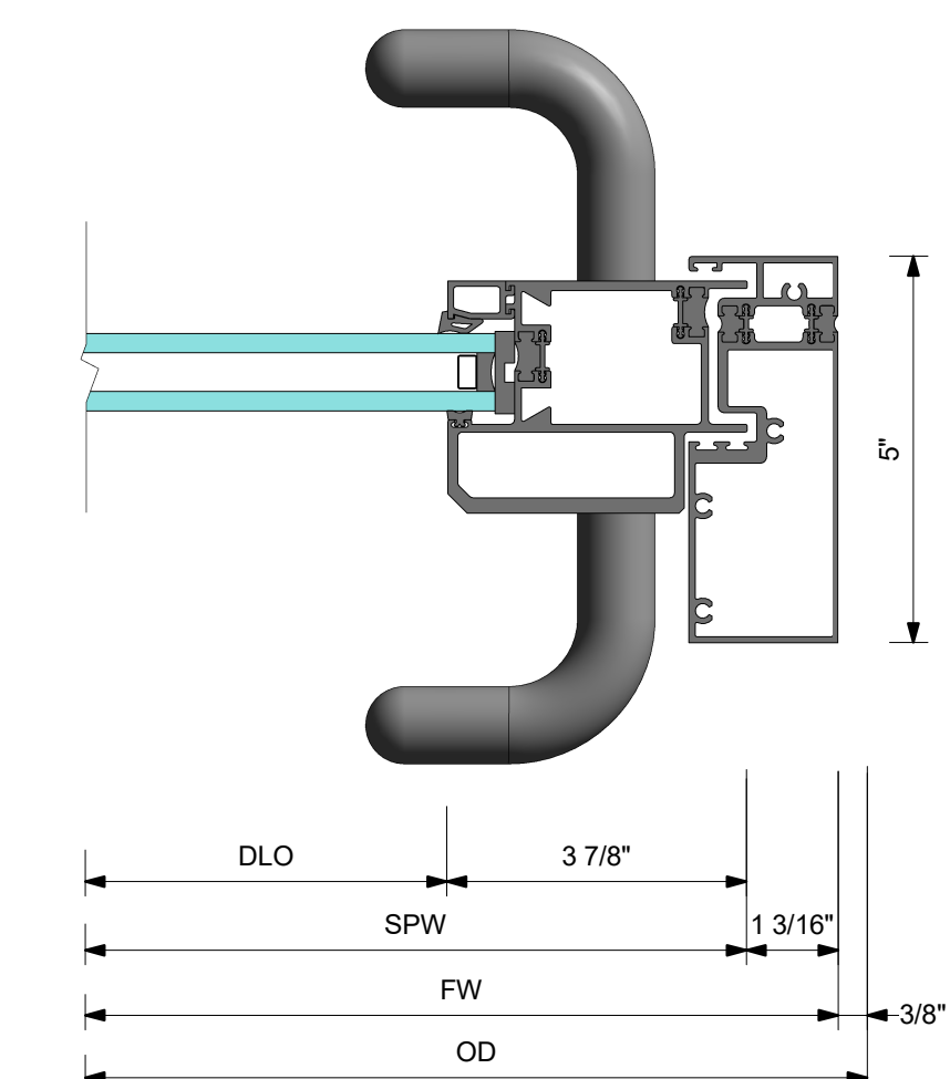
7 DETAIL 7 VERTICAL OX JAMB WITH CO-9 PULL SLIDING PANEL STILE
