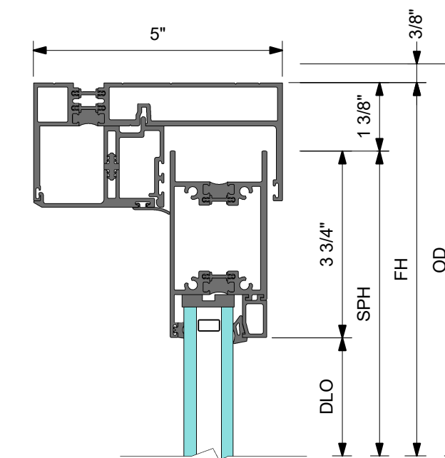
1 DETAIL 1 HEAD AT SLIDING PANEL
