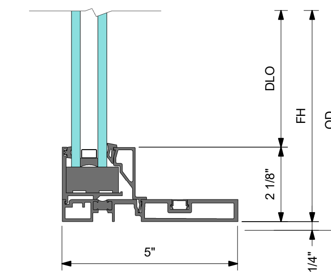
4 DETAIL 4 LOW PROFILE SILL AT FIXED PANEL
