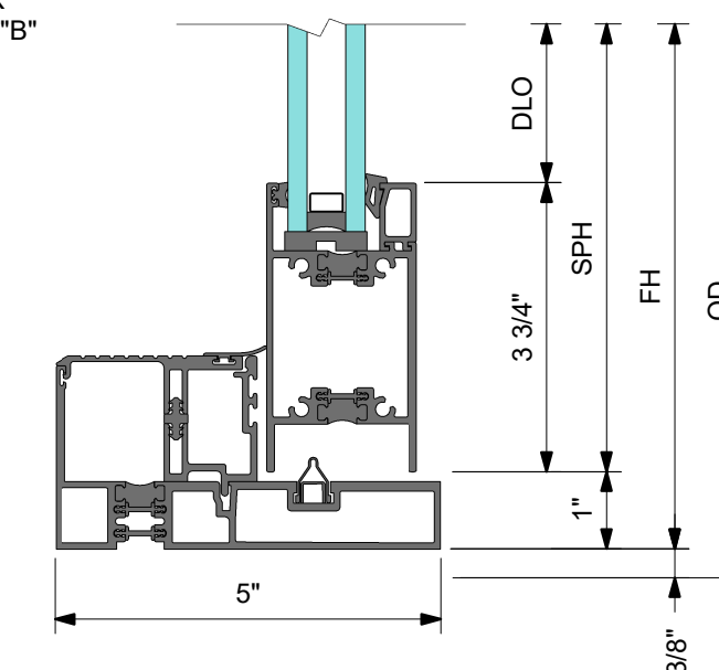
3 DETAIL 2 SILL AT SLIDING PANEL
