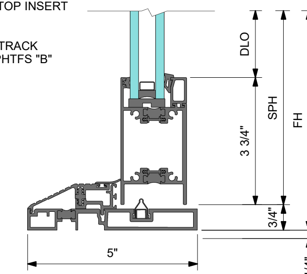
3 DETAIL 2 LOW PROFILE SILL AT SLIDING PANEL
