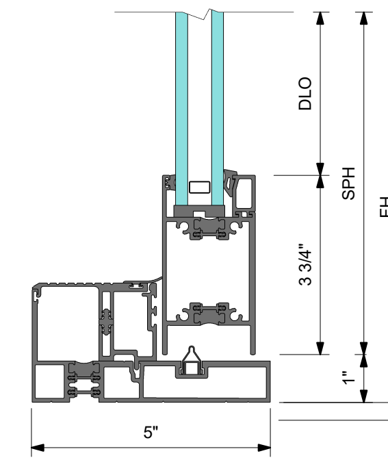
2 DETAIL 2 SILL AT SLIDING PANEL
