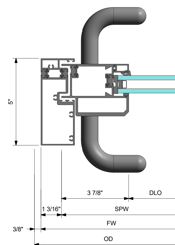
5 DETAIL 5 VERTICAL XO JAMB WITH CO-9 PULL SLIDING PANEL STILE
