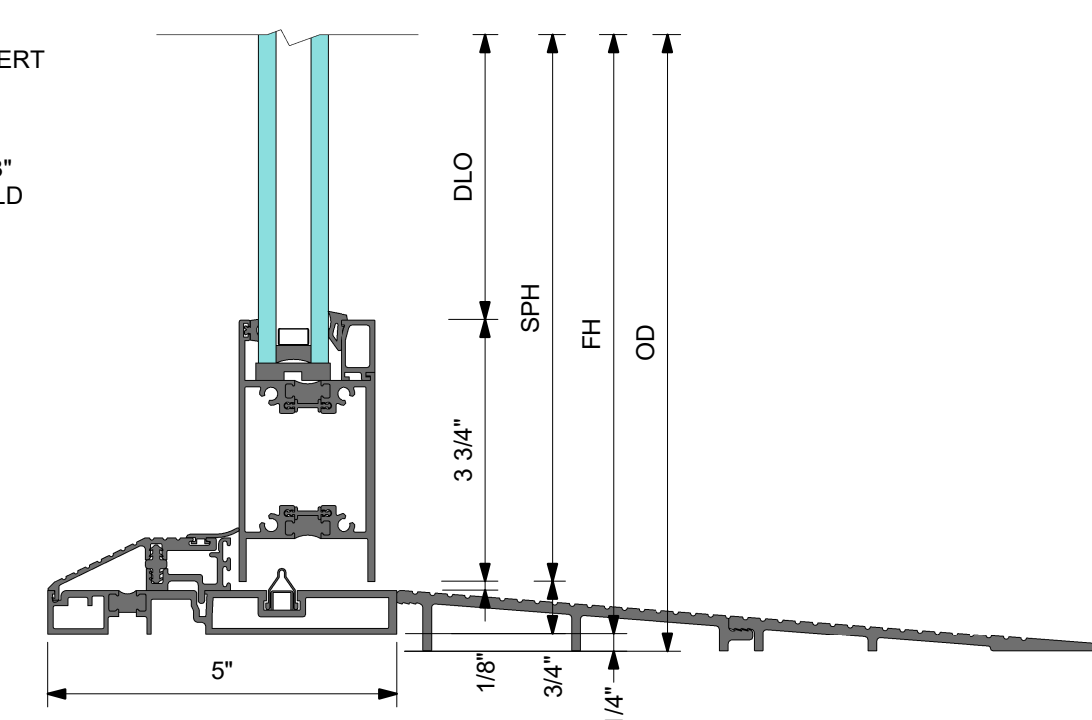
2 DETAIL 2 LOW PROFILE SILL WITH RAMP AT SLIDING PANEL
