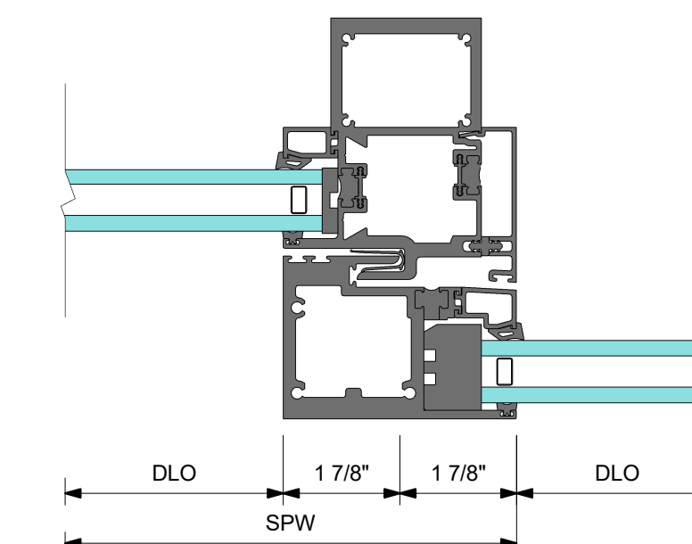
6 DETAIL 6 VERTICAL OX INTERMEDIATE FIXED SLIDING WITH STANDARD INTERLOCK
