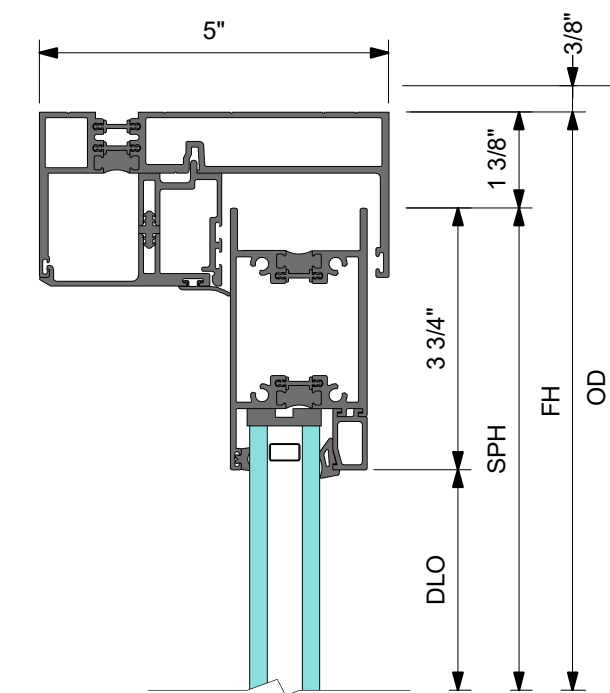
1 DETAIL 1 HEAD AT SLIDING PANEL
