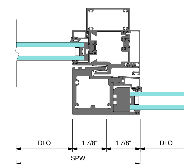
6 DETAIL 6 VERTICAL XO INTERMEDIATE FIXED SLIDING WITH STANDARD INTERLOCK
