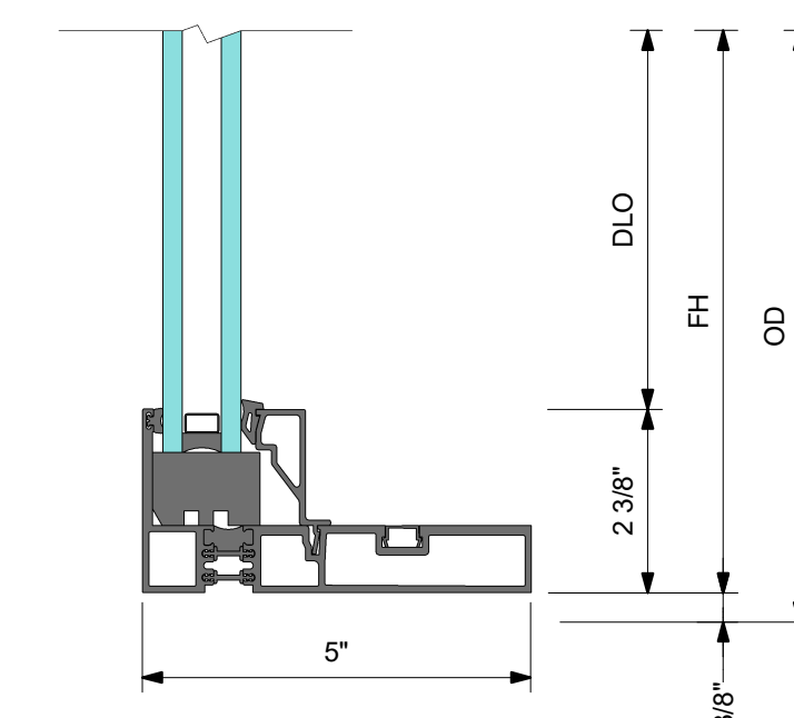
4 DETAIL 4 SILL AT FIXED PANEL
