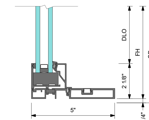
4 DETAIL 4 LOW PROFILE SILL AT FIXED PANEL
