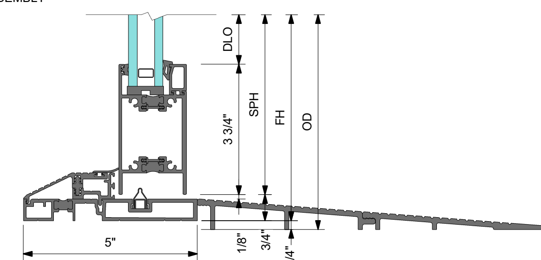
2 DETAIL 2 LOW PROFILE SILL WITH RAMP AT SLIDING PANEL
