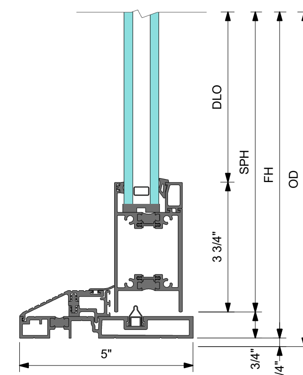
2 DETAIL 2 LOW PROFILE SILL AT SLIDING PANEL
