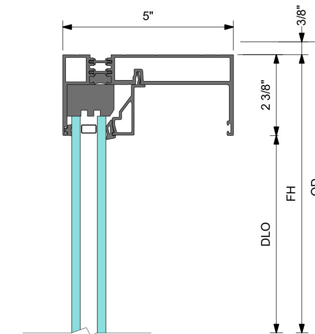
3 DETAIL 3 HEAD AT FIXED PANEL
