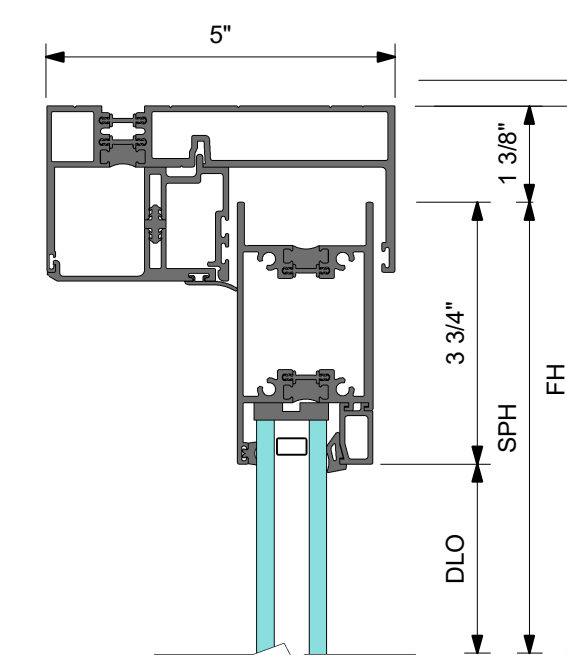
1 DETAIL 1 HEAD AT SLIDING PANEL
