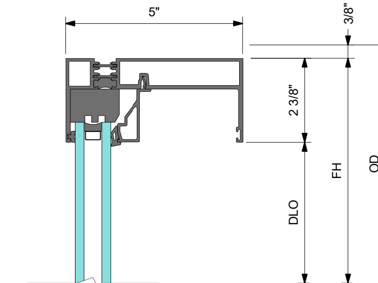
3 DETAIL 3 HEAD AT FIXED PANEL
