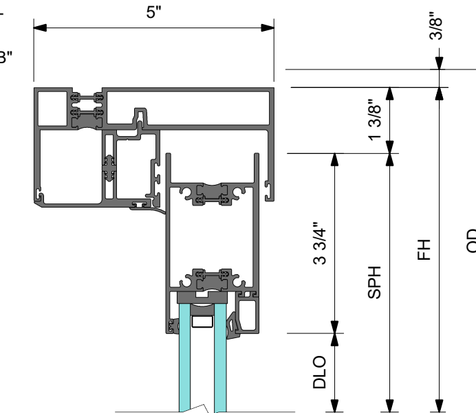
1 DETAIL 1 HEAD AT SLIDING PANEL
