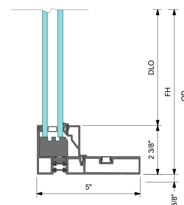
4 DETAIL 4 SILL AT FIXED PANEL
