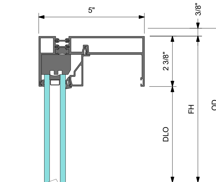
3 DETAIL 3 HEAD AT FIXED PANEL
