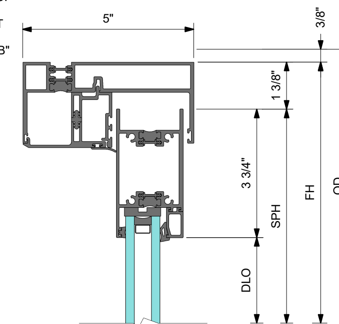
1 DETAIL 1 HEAD AT SLIDING PANEL
