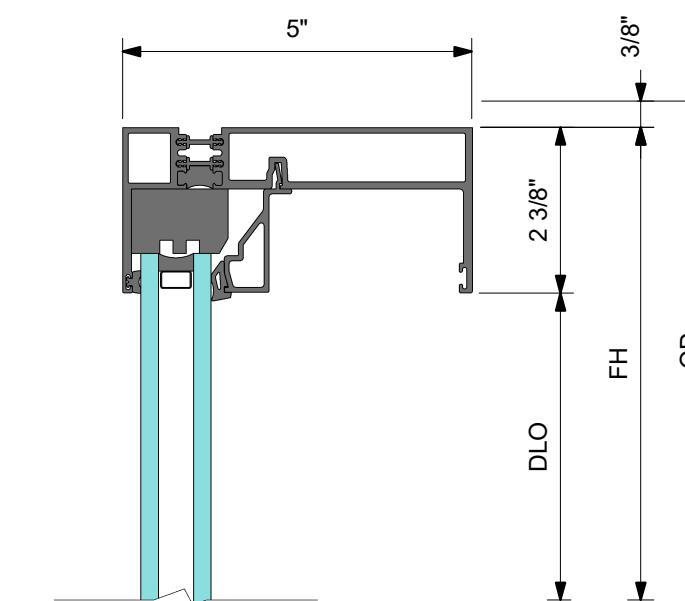
3 DETAIL 3 HEAD AT FIXED PANEL
