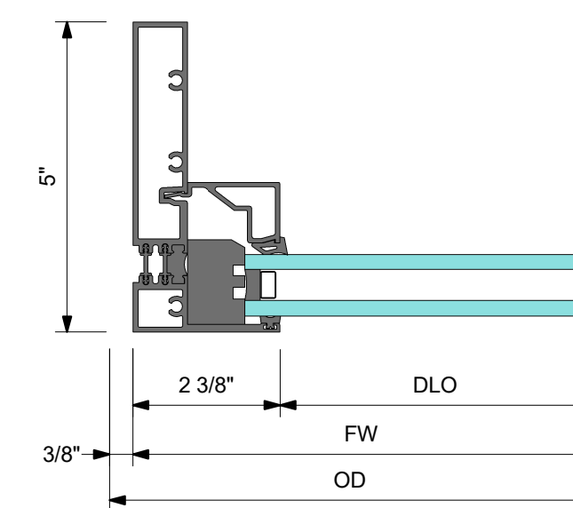
5 DETAIL 5 VERTICAL OX JAMB FIXED PANEL
