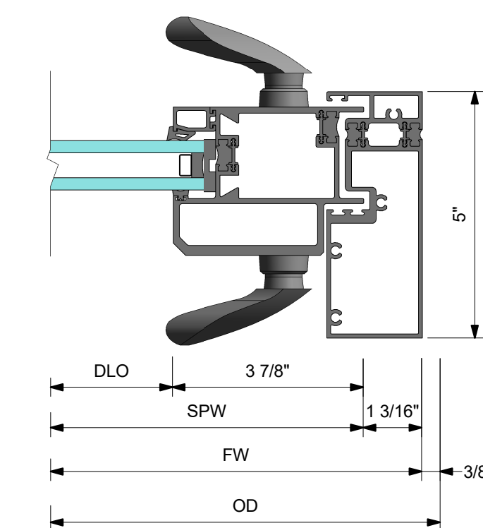
7 DETAIL 7 VERTICAL OX JAMB WITH STANDARD PULL SLIDING PANEL STILE
