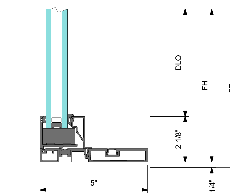
4 DETAIL 4 LOW PROFILE SILL AT FIXED PANEL
