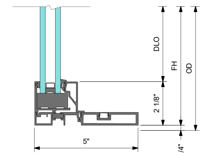
4 DETAIL 4 LOW PROFILE SILL AT FIXED PANEL
