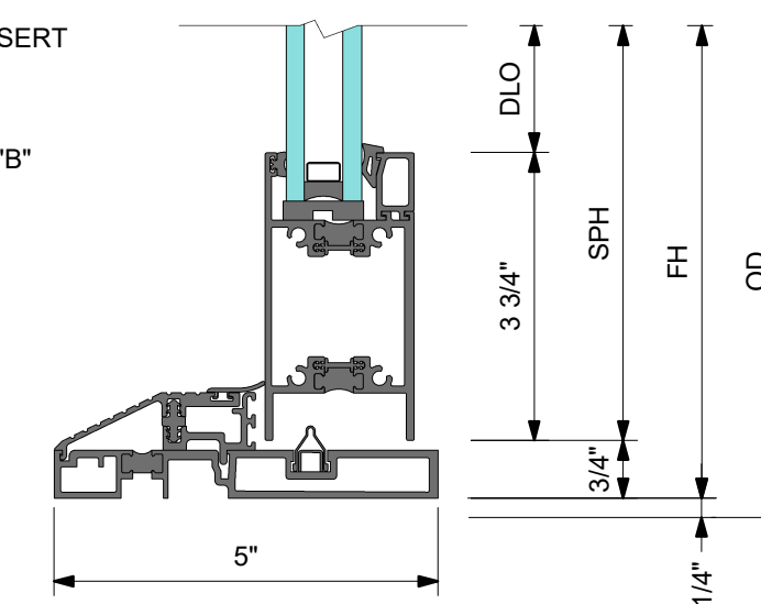
2 DETAIL 2 LOW PROFILE SILL AT SLIDING PANEL
