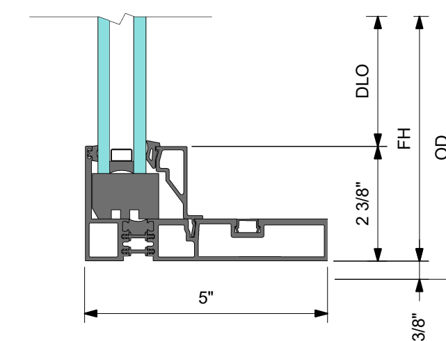
4 DETAIL 4 SILL AT FIXED PANEL
