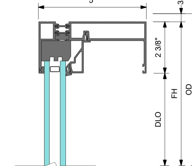
3 DETAIL 3 HEAD AT FIXED PANEL
