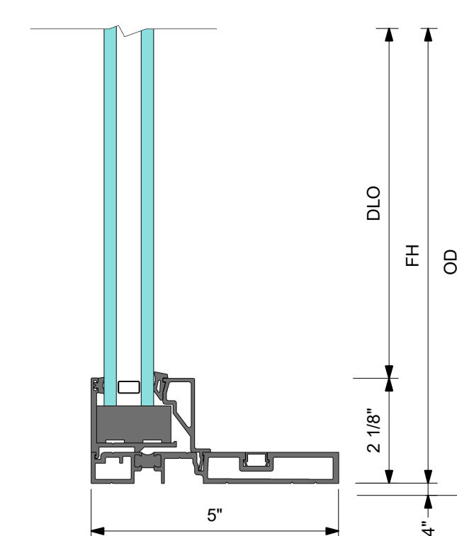
4 DETAIL 4 LOW PROFILE SILL AT FIXED PANEL
