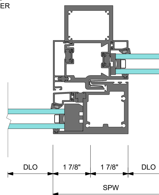
6 DETAIL 6 VERTICAL OX INTERMEDIATE FIXED SLIDING WITH STANDARD INTERLOCK
