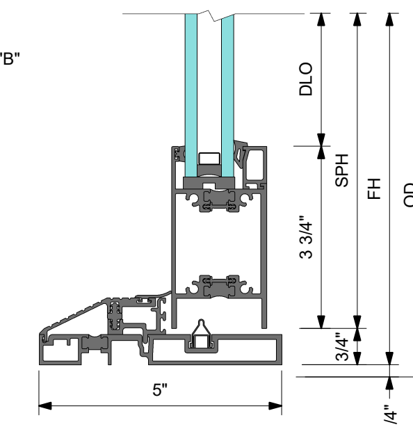
2 DETAIL 2 LOW PROFILE SILL AT SLIDING PANEL
