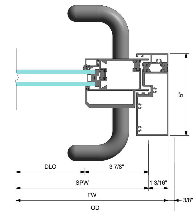
7 DETAIL 7 VERTICAL OX JAMB WITH CO-9 PULL SLIDING PANEL STILE
