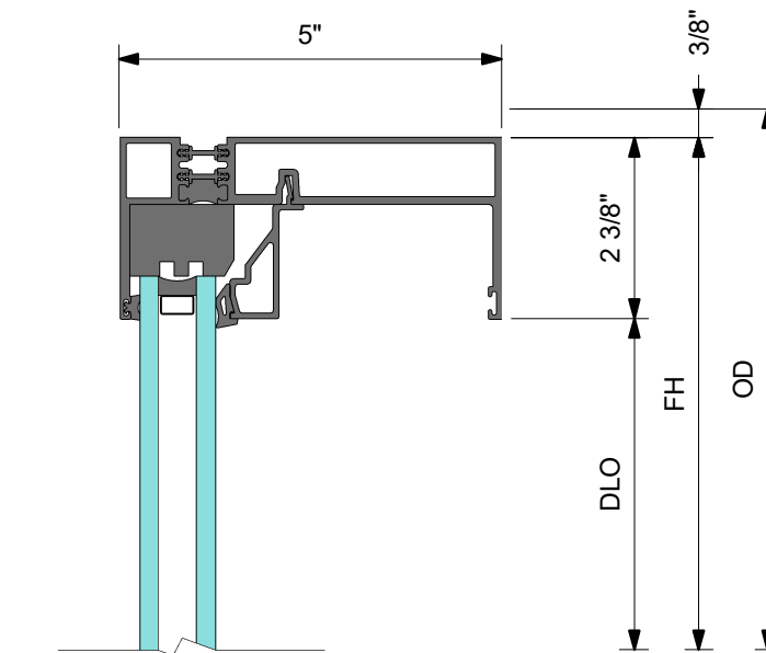
2 DETAIL 3 HEAD AT FIXED PANEL
