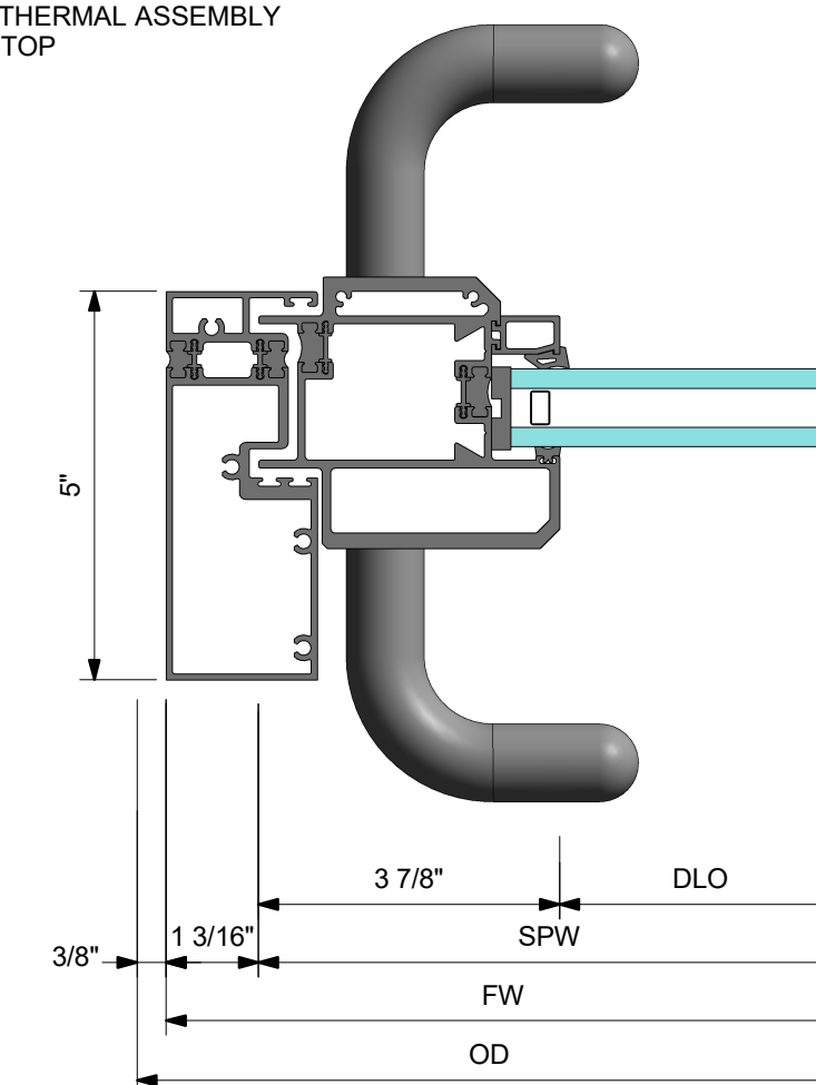
5 DETAIL 5 VERTICAL XO JAMB WITH CO-9 PULL SLIDING PANEL STILE
