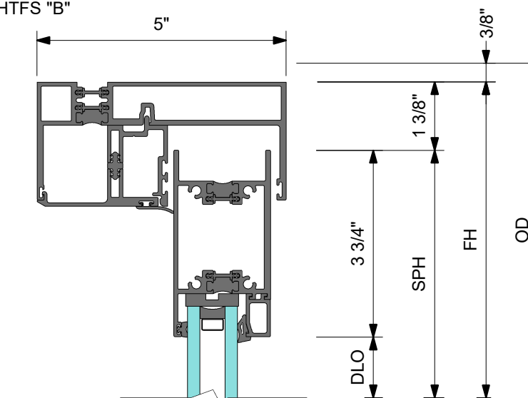
1 DETAIL 1 HEAD AT SLIDING PANEL
